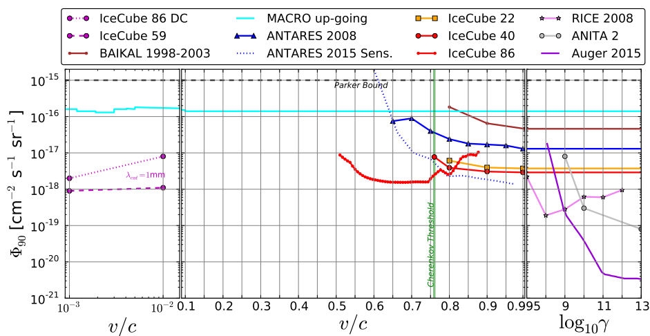
Figure 1. 90% CL upper limits versus velocity \beta for a flux of very energetic cosmic GUT monopoles with magnetic charge of g = g_D . The IceCube 86 DC nucleon-decay analysis is based on the IceCube DeepCore [61]. Results from MACRO [49], ANTARES [57], RICE [63], BAIKAL [55], ANITA [64], and Auger [65] are superimposed on IceCube limits from direct (IceCube 40) [59] and indirect (IceCube 86) Cherenkov light [60]—from Ref. [62].
