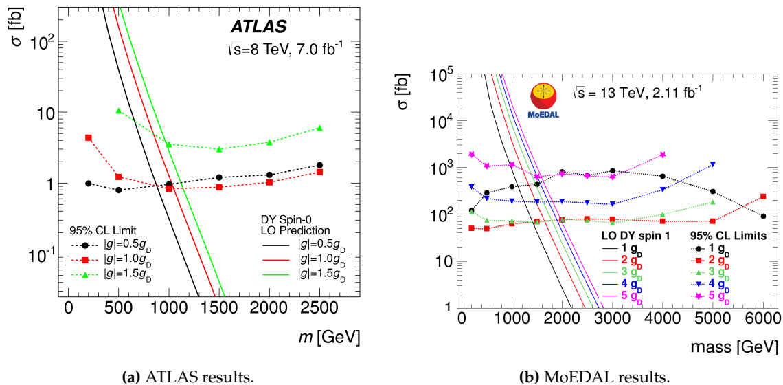
Figure 2. (a) 95% cross-section upper limits (dashed lines) and theoretical cross sections (solid lines) for magnetic monopoles with spin 0 and various magnetic charges—from Ref. [88]; (b) cross-section upper limits at 95% confidence level for DY monopole production as a function of mass for spin-1 monopoles. The various line colours correspond to different monopole charges. The solid lines represent DY cross-section calculations at leading order. From Ref. [92].
